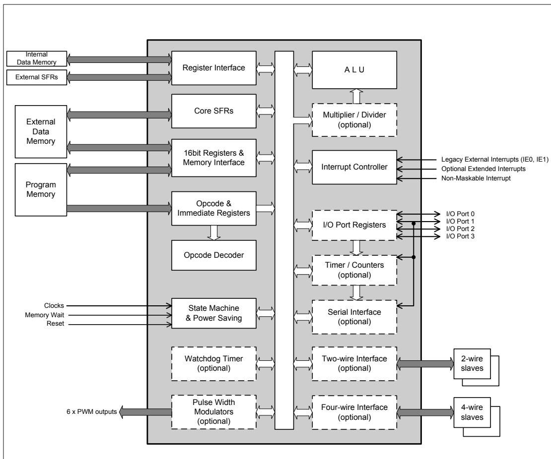
M8051W Architecture
